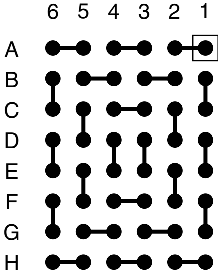
BALL VIEW
